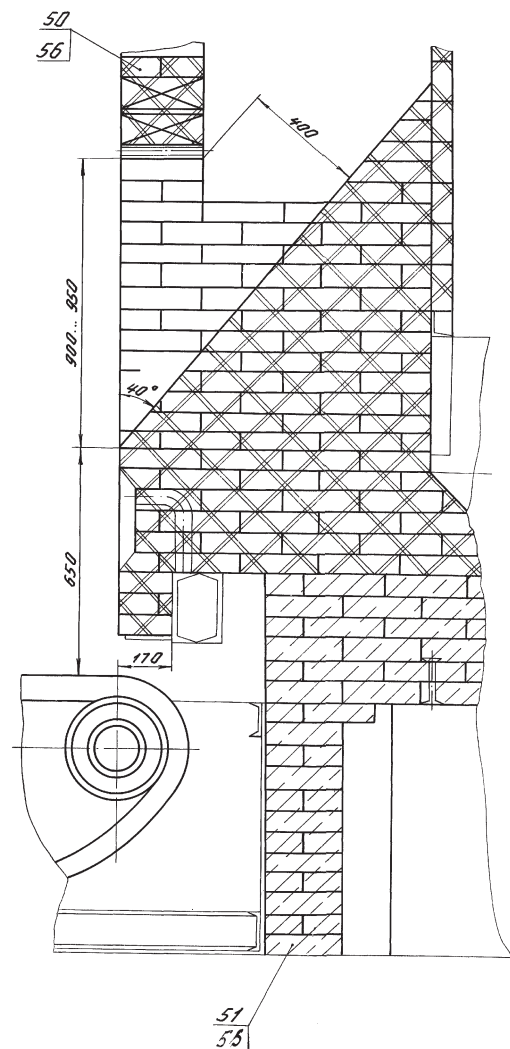
3-3 (1:10) (1)
